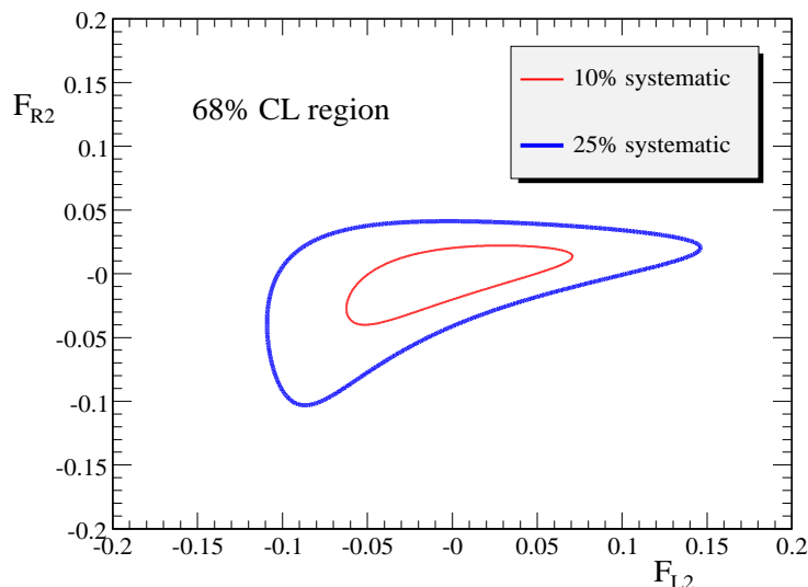
Figure 4: The 68% confidence level regions of anomalous couplings with 10% and 25% of systematic uncertainties.
